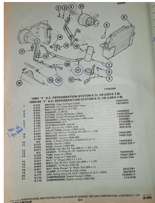
Manual diagram of the complete A/C system.
